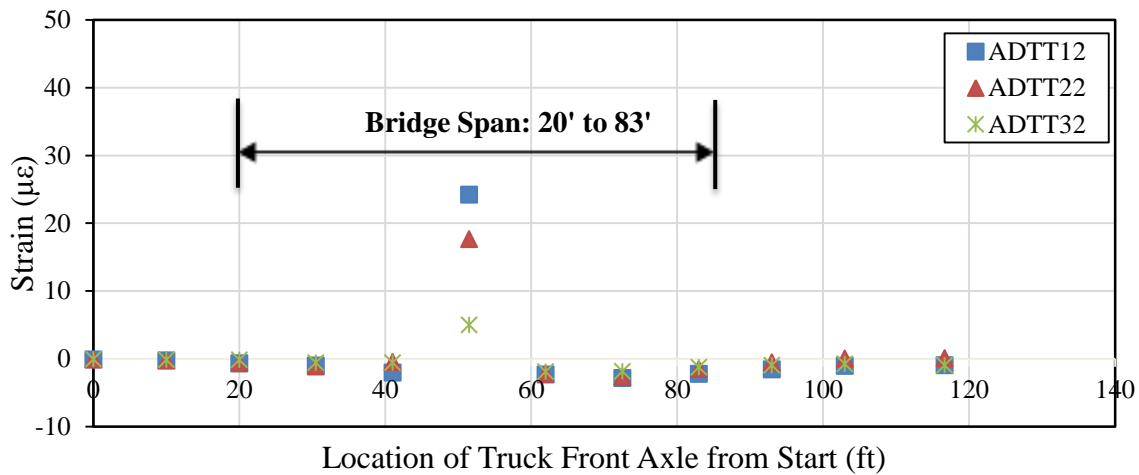
Figure 4.16. Transverse top strains at end panel for load path 2
