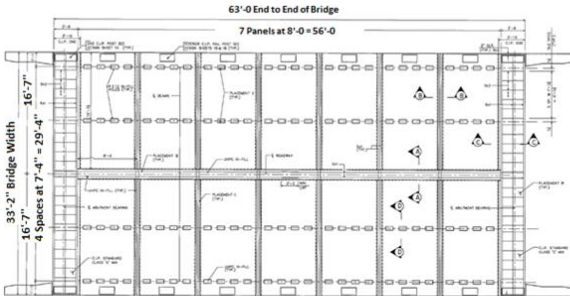
Figure 2.1. Plan of the UHPC waffle deck bridge in Wapello County, Iowa
