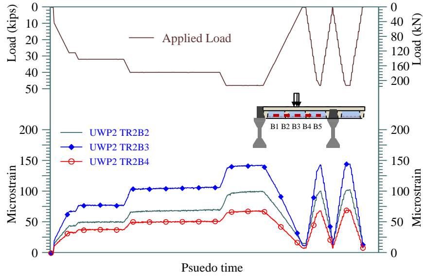
Figure 2.32. Measured strains in the bottom reinforcement of transverse rib TR2 along the length of panel UWP2 at the overload load
