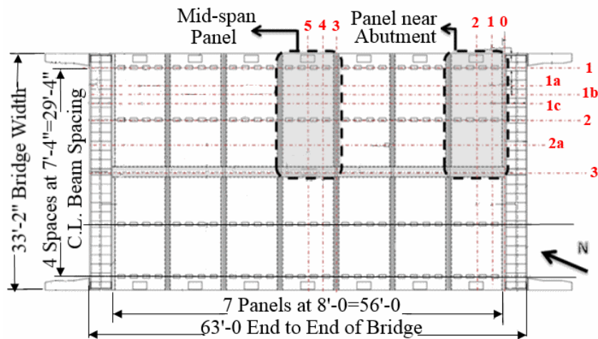
Figure 4.1. Dahlonga road bridge plan
