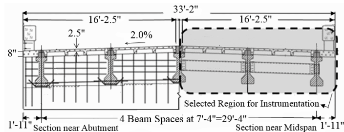
Figure 4.2. Dahlonga road bridge cross section
