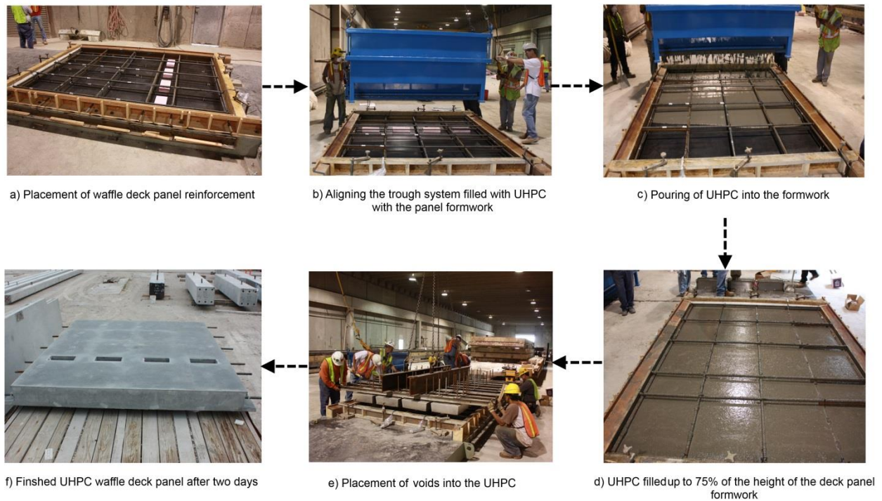
Figure 2.9. Construction sequence used for the UHPC waffle deck panels at the precast plant
