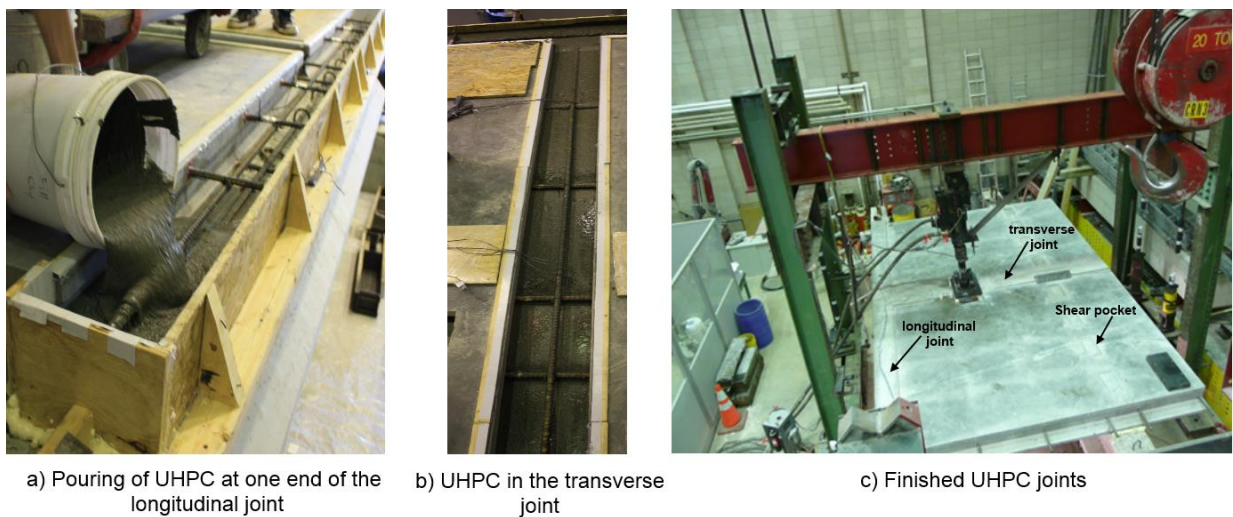
Figure 2.12. Construction of UHPC joints in the ISU laboratory
