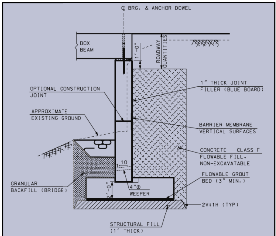
Fig. 6. Abutment section.
