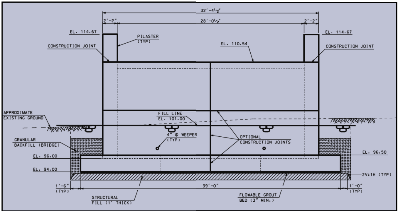
Fig. 5. Abutment elevation.
