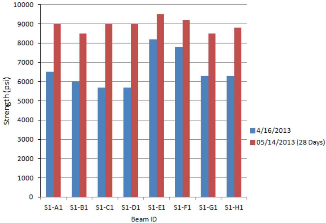
Figure 15: 28-Day Compressive Concrete Strength Development
