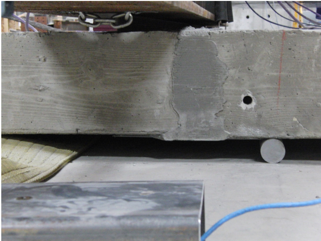
Figure 25: Shear Reactions.
