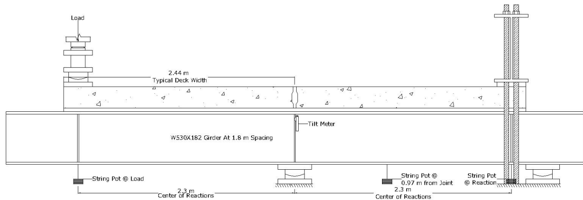
Figure 9: Full-Scale Testing Setup.
