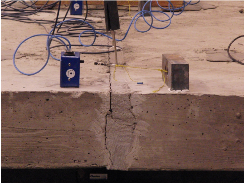
Figure 30: Cracking Along Joint.
