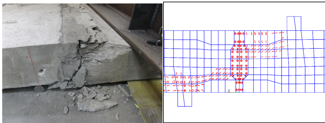
Figure 6: Shear Failure (Test Specimen and ANSYS Models).
