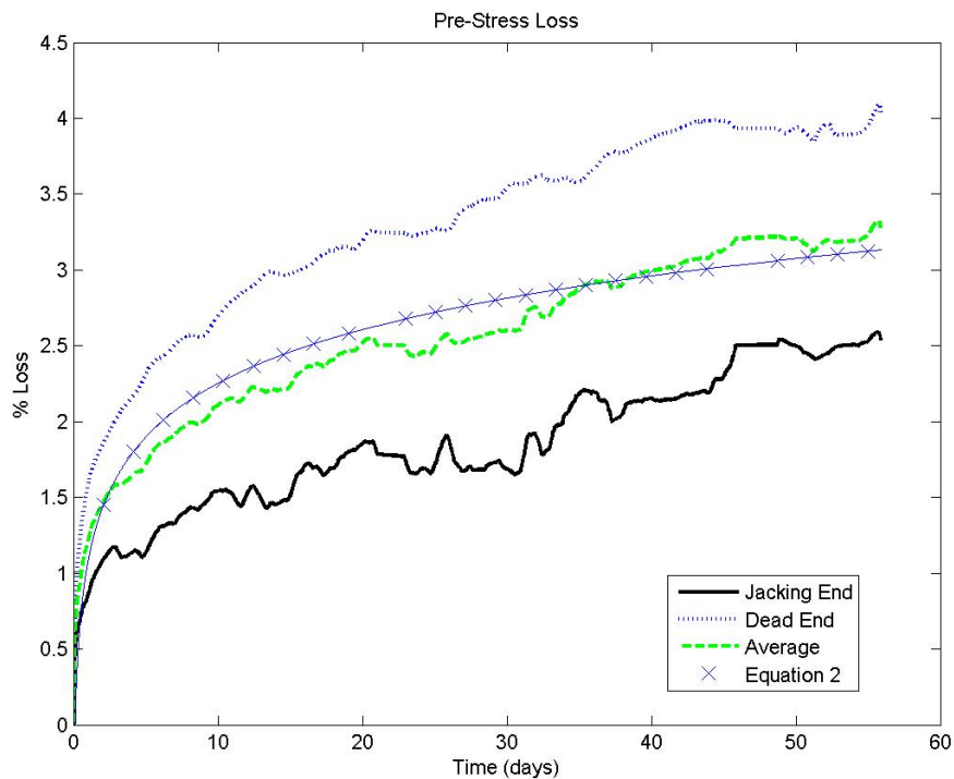
Figure 7: Pre-Stress Loss vs. Time.
