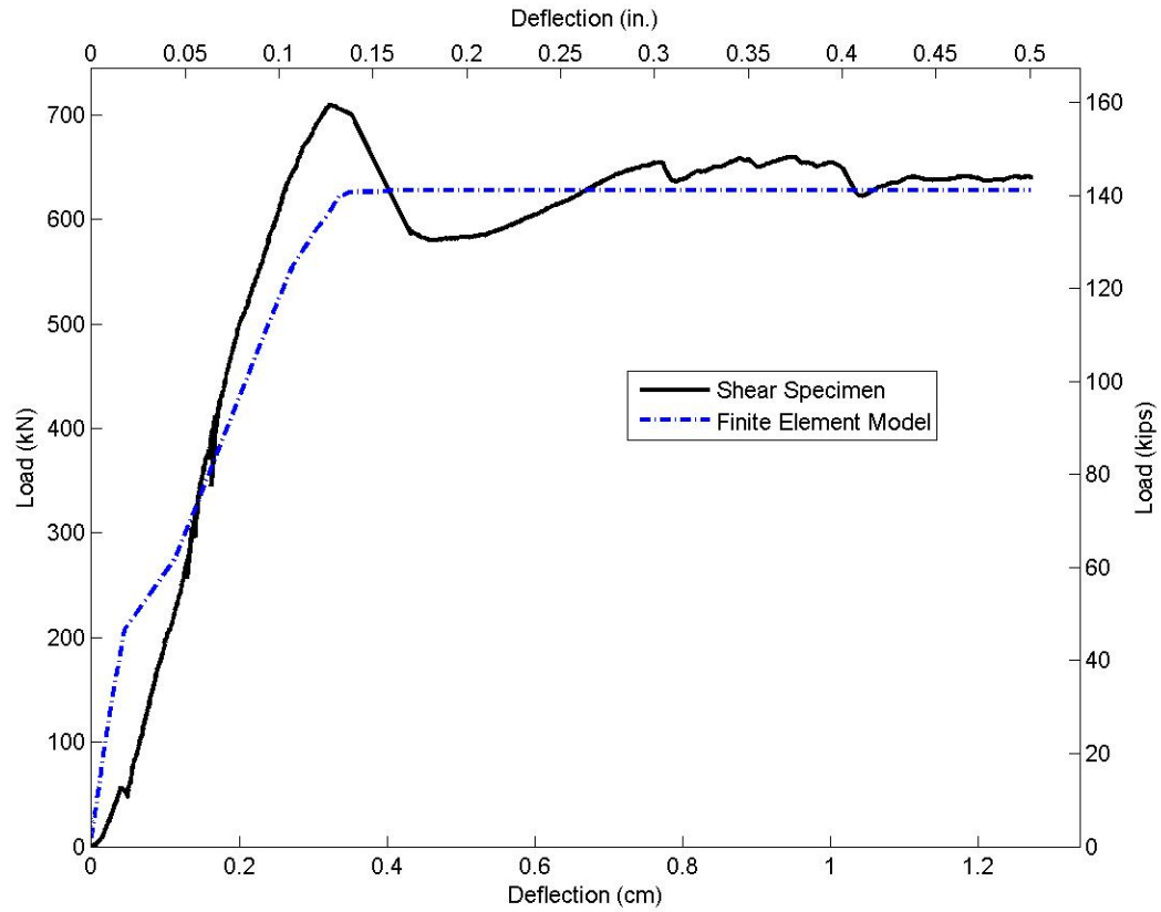
Figure 5: Load vs. Deflection Shear Specimen.
