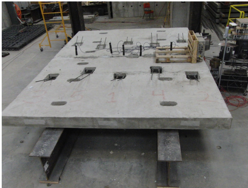
Figure 8: Layout of Full-Scale Specimen Prior to Grouting.
