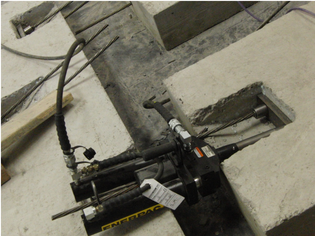
Figure 19: Post-Tensioning.
