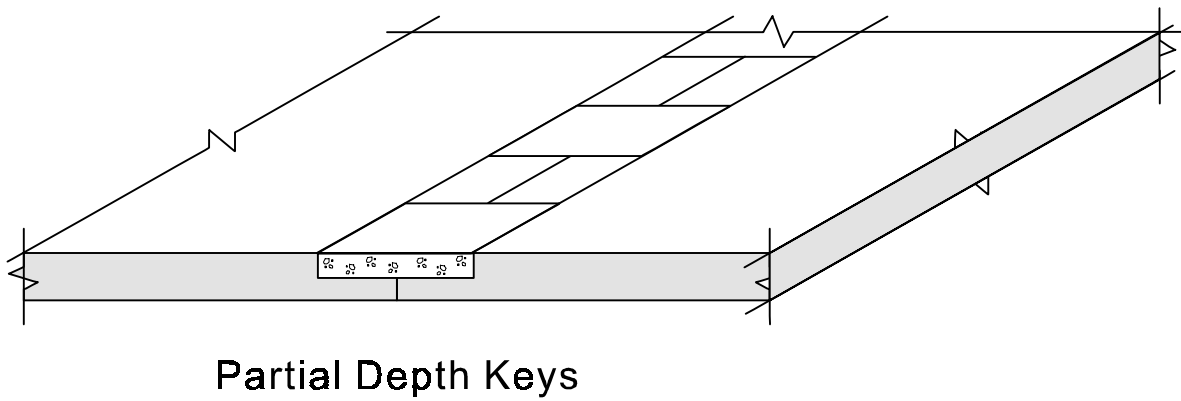
Figure 19. Connection Details for Joining of Flanges in Double Tees.
