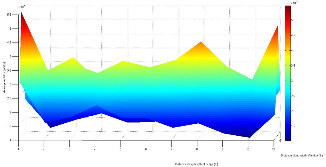
Fig 11. 3-D Mobility Plot, Mass 14 detail.
